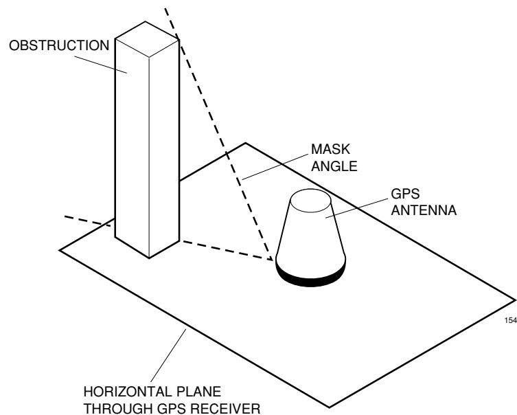
Figure 2-1. Mask Angle Definition
